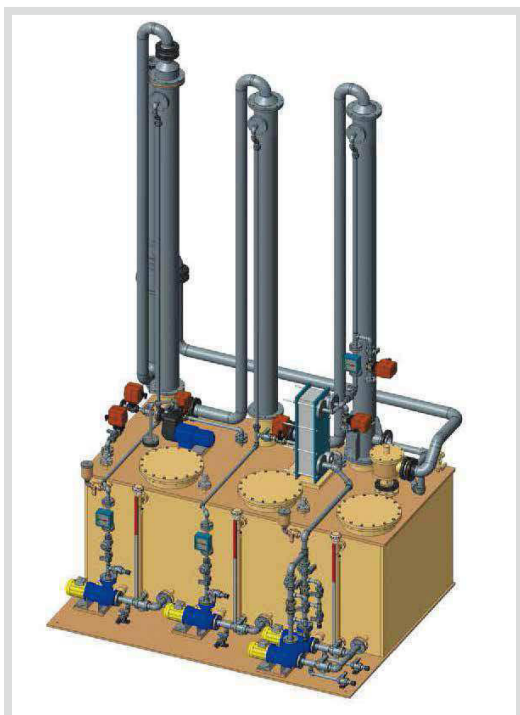
Multistage packed column EO Scrubber
